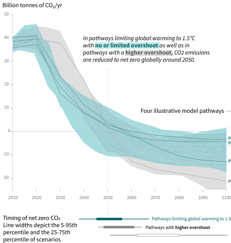
Figure SPM.3a | Global emissions pathway characteristics. The main panel shows global net anthropogenic CO 2 emissions in pathways limiting global warming to 1.5°C with no or limited (less than 0.1°C) overshoot and pathways with higher overshoot. The shaded area shows the full range for pathways analysed in this Report. The panels on the right show non-CO 2 emissions ranges for three compounds with large historical forcing and a substantial portion of emissions coming from sources distinct from those central to CO 2 mitigation. Shaded areas in these panels show the 5–95% (light shading) and interquartile (dark shading) ranges of pathways limiting global warming to 1.5°C with no or limited overshoot. Box and whiskers at the bottom of the figure show the timing of pathways reaching global net zero CO 2 emission levels, and a comparison with pathways limiting global warming to 2°C with at least 66% probability. Four illustrative model pathways are highlighted in the main panel and are labelled P1, P2, P3 and P4, corresponding to the LED, S1, S2, and S5 pathways assessed in Chapter 2. Descriptions and characteristics of these pathways are available in Figure SPM.3b. {2.1, 2.2, 2.3, Figure 2.5, Figure 2.10, Figure 2.11}
